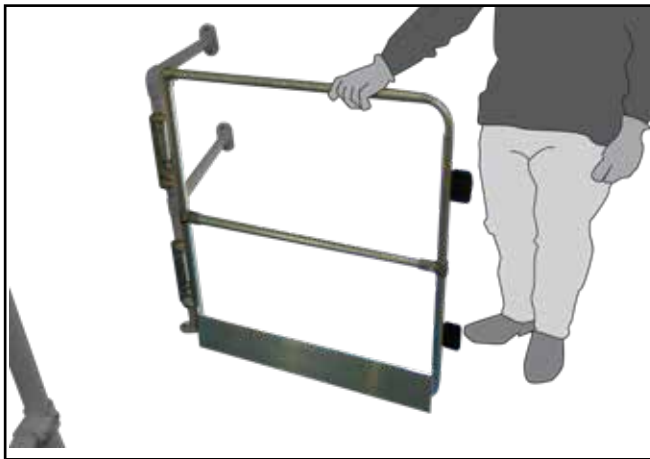
S. Manually open the gate at 45 degrees from its closed position.
